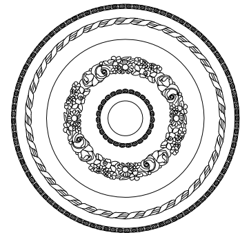
PLAS 923 FLORAL WREATH ROSETTE 27-1/2" DIAMETER x 1-11/16" DEPTH 4-3/16" DIAMETER AT CENTER HOLE 1-11/16" DEPTH AT CENTER 6-1/8" DIA. FLAT AREA AT CENTER 15 LBS TOTAL WEIGHT (RMF 7045 IS FLORAL BAND)
